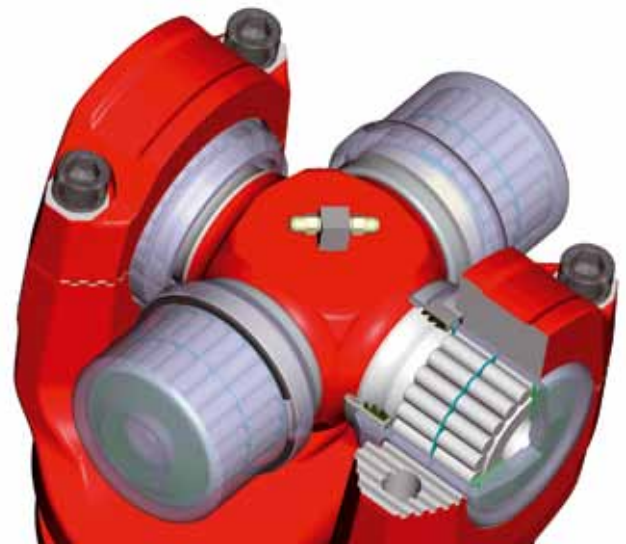
▲ Split bearing eye
