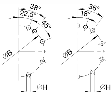
8-hole flange
