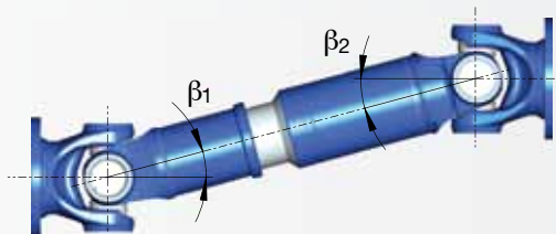
Z-arrangement
