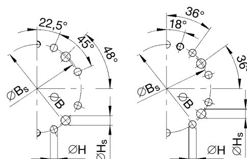
8-hole flange
