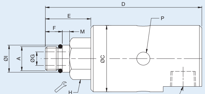
Radial Connection (1115 series)
